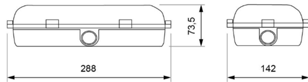
Watertight mounting
